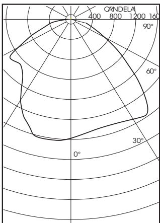
Report No.: LL02504 Four 32 watt T8 fluorescent lamps 24 inch Asymmetric Lens in white painted troffer
