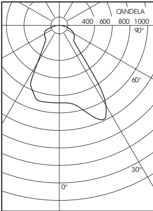
Report No.: LL02527 Single 32 watt T8 Fluorescent 12 inch Asymmetric Lens in white painted troffer
