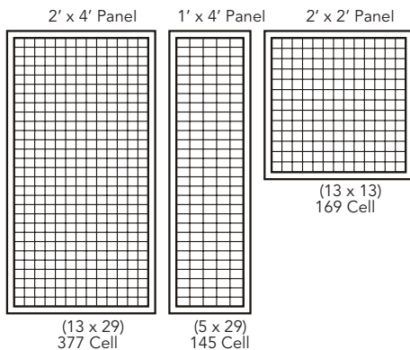
Kwik-Fit PLMA Cell Configuration
