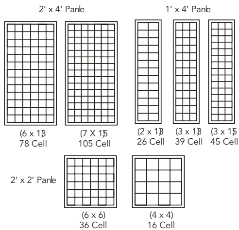
Kwik-Fit PLLA Cell Configuration
